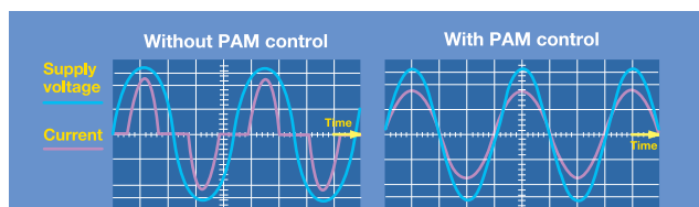
PAM adjusts the form of the current wave so that it becomes close to that of the supply voltage wave. High harmonics are reduced and 98% of the electricity is utilized.
